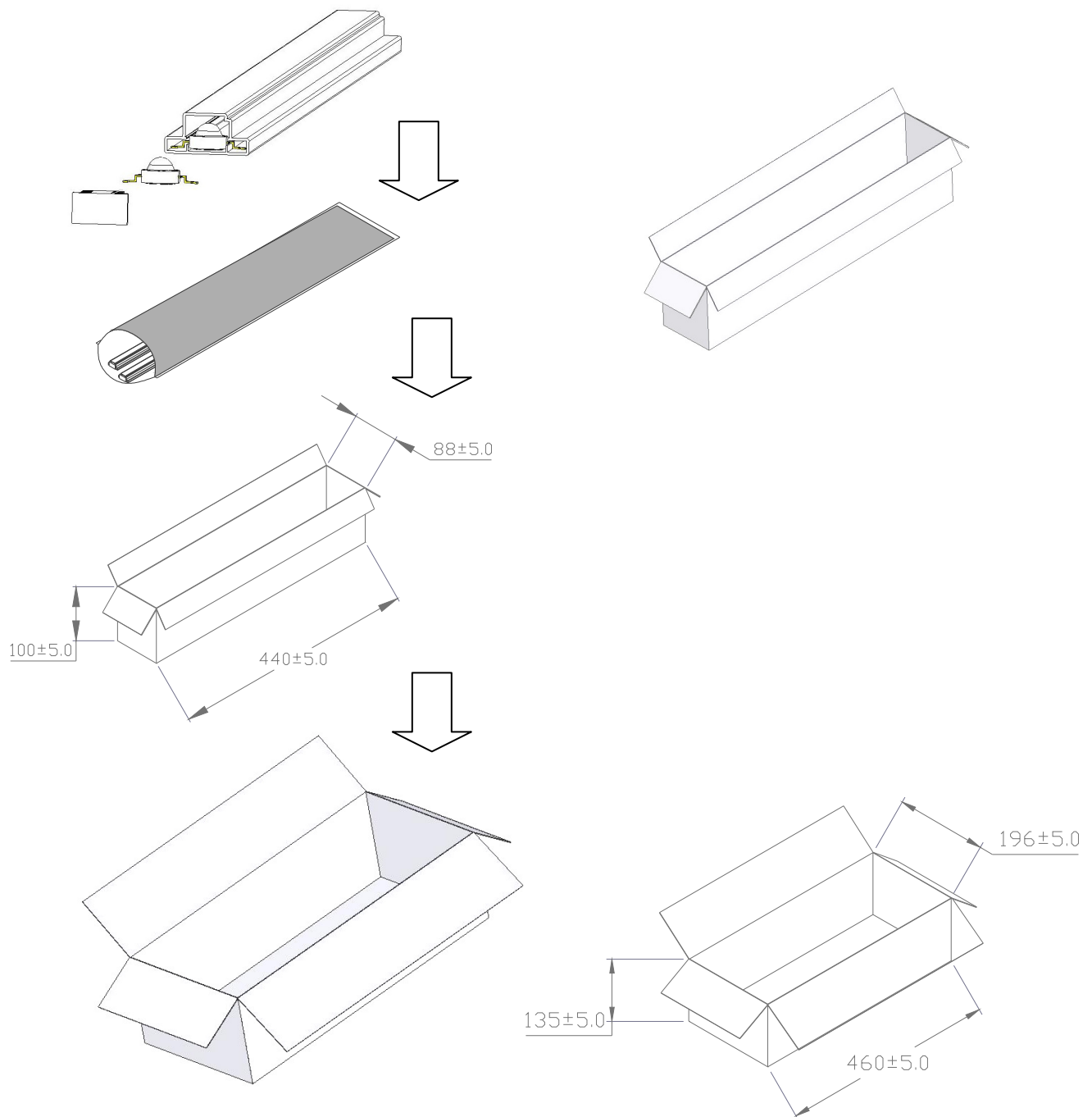
< Figure 8 Package steps and dimensions >
