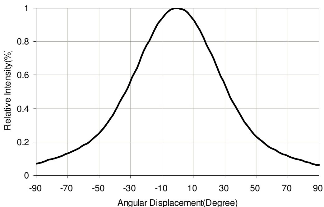
< Figure 4.Lambertain at T_J=25^{\circ}\text{C} for cool white, neutral white, and warm white >
