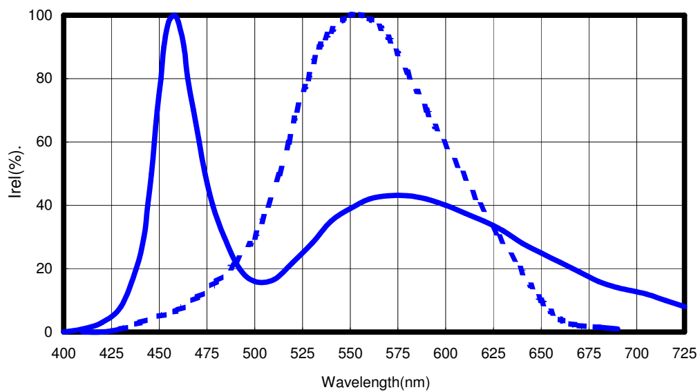
<Figure 2 Cool white color spectrum at T_j = 25^\circ\text{C} .for Edixeon ® series >
