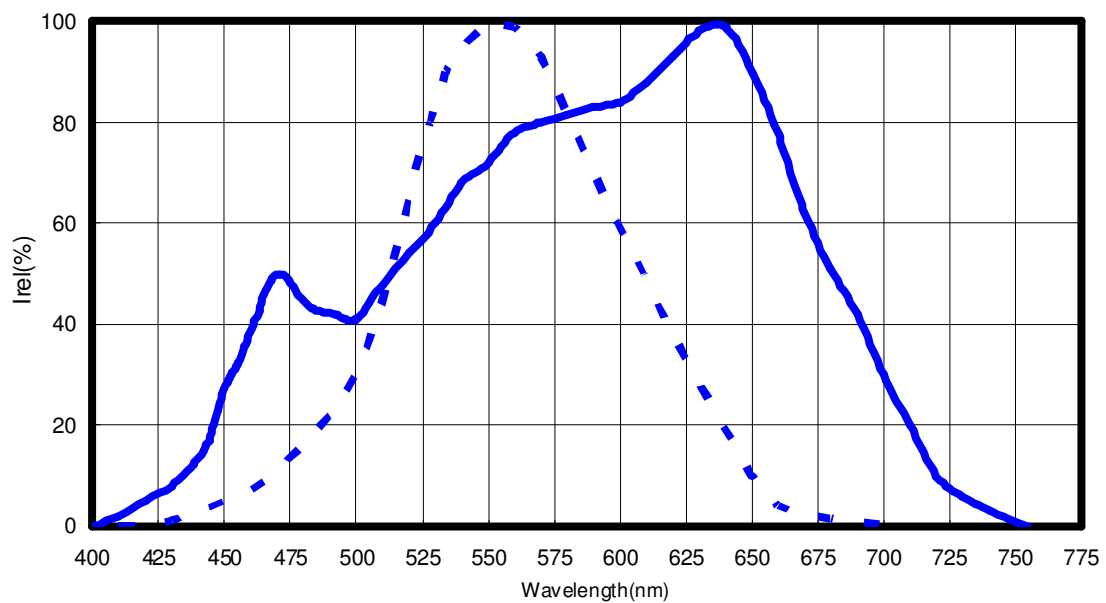
< Figure 3 Neutral white and warm white color spectrum at T_j = 25^\circ\text{C} . for Edixeon ® 1NA5 series >
